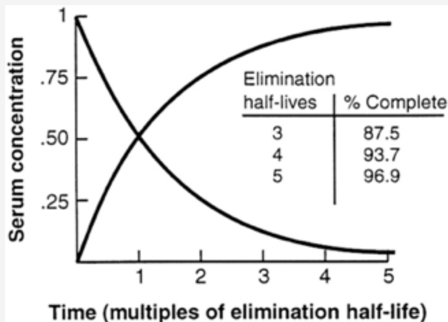
Figure 1: Half-lives required to achieve steady-state and complete drug elimination
